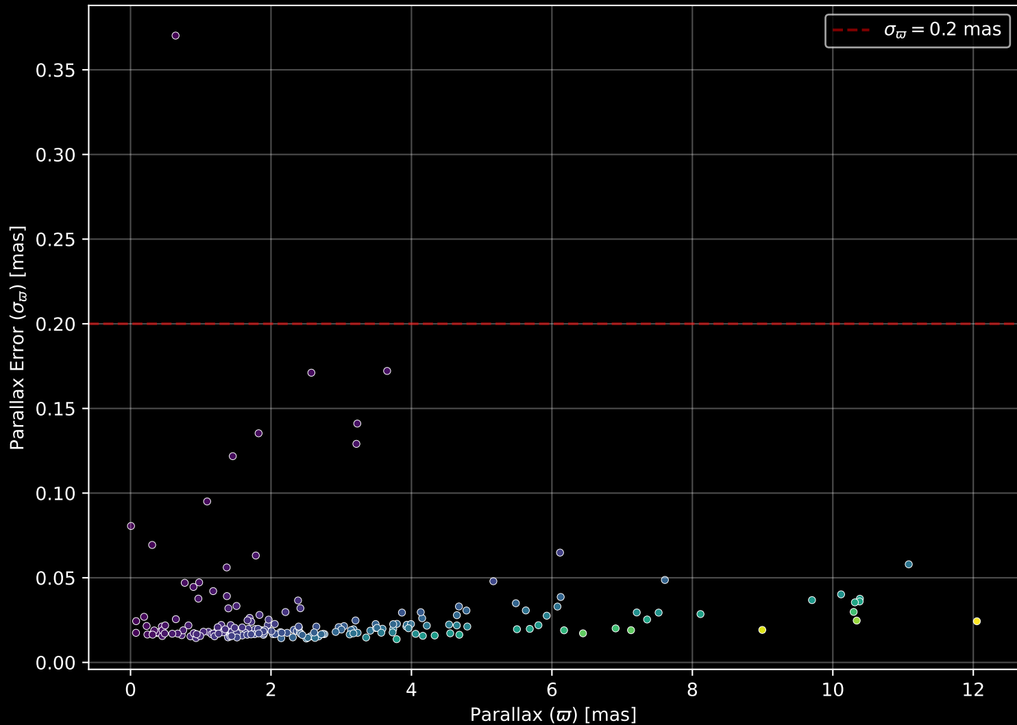
APOGEE DR17 Field: [K2EB_C06_320+48_btx] Parallax Quality (n= 197)
