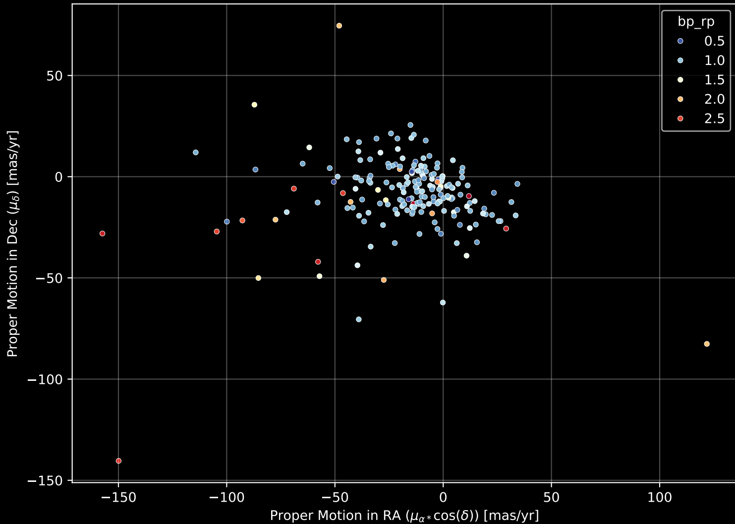
APOGEE DR17 Field: [K2EB_C06_320+48_btx] Proper Motion Diagram (n= 197)
