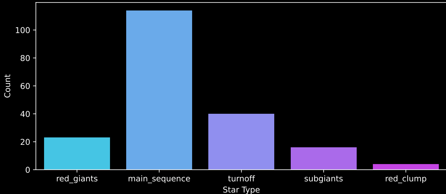
APOGEE DR17 Field: [K2EB_C06_320+48_btx] Count plot of Star Type
