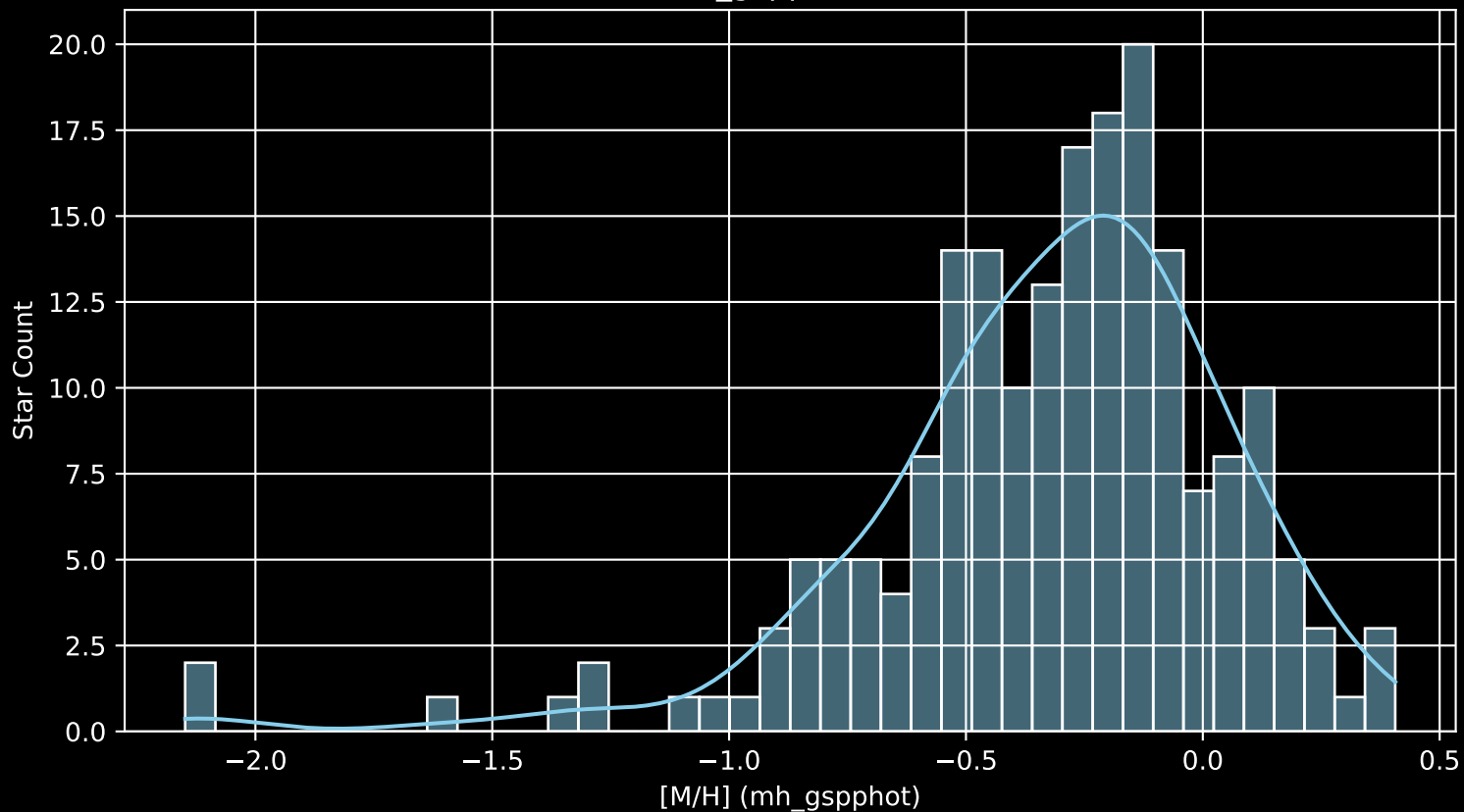
APOGEE DR17 Field: [K2EB_C06_320+48_btx [M/H] (mh_gspphot) (n= 196)
