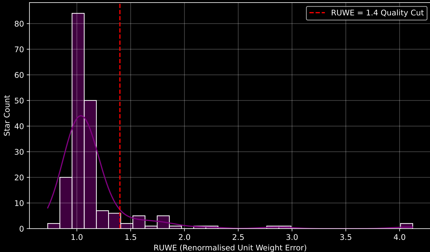
GAPOGEE DR17 Field [K2EB_C06_320+48_btx] RUWE Distribution (n= 189)
