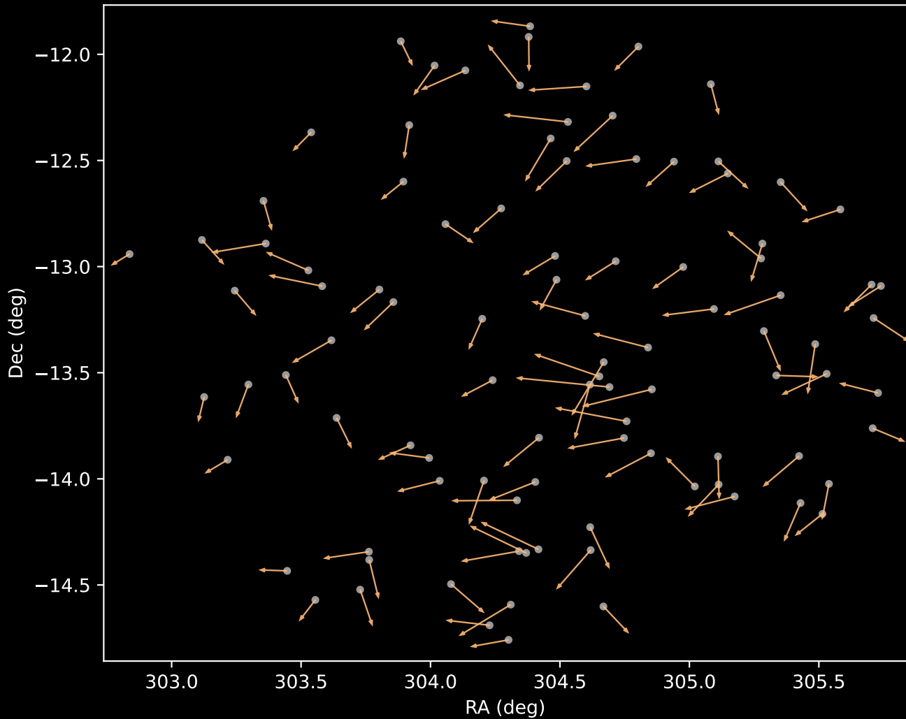
APOGEE DR17 Cluster 3 Proper Motion Vectors (n=98)
